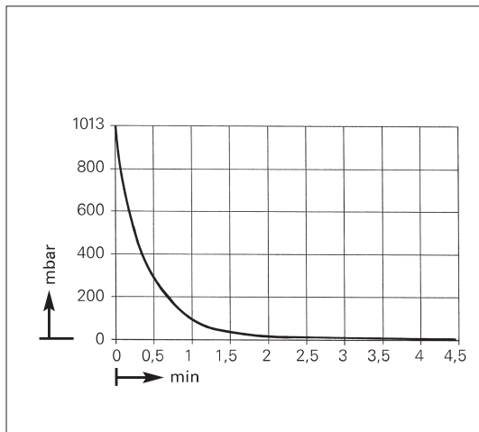
Pump down time for 20 l receiver
