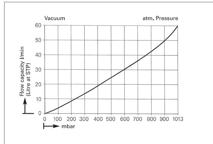
Performance characteristics
