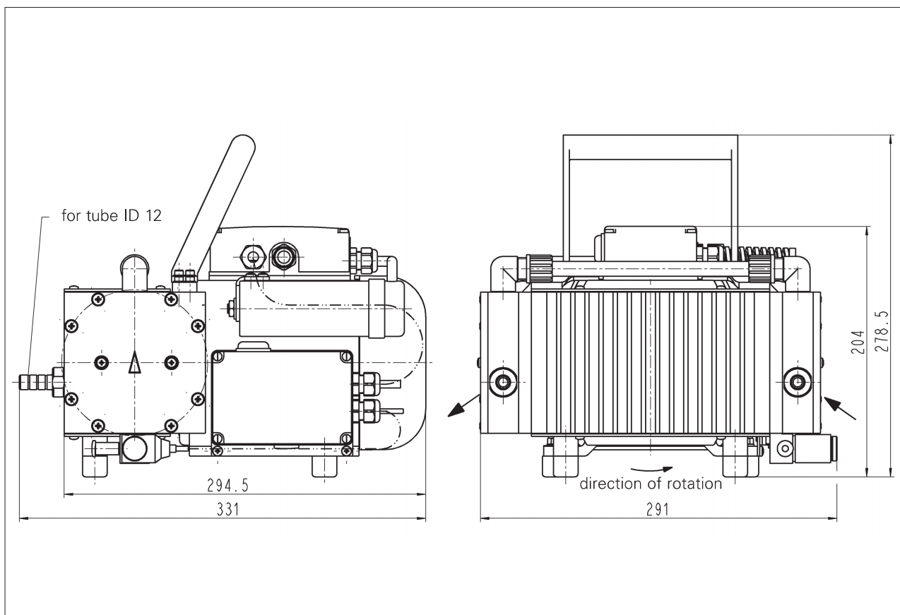
Dimensions (mm)
