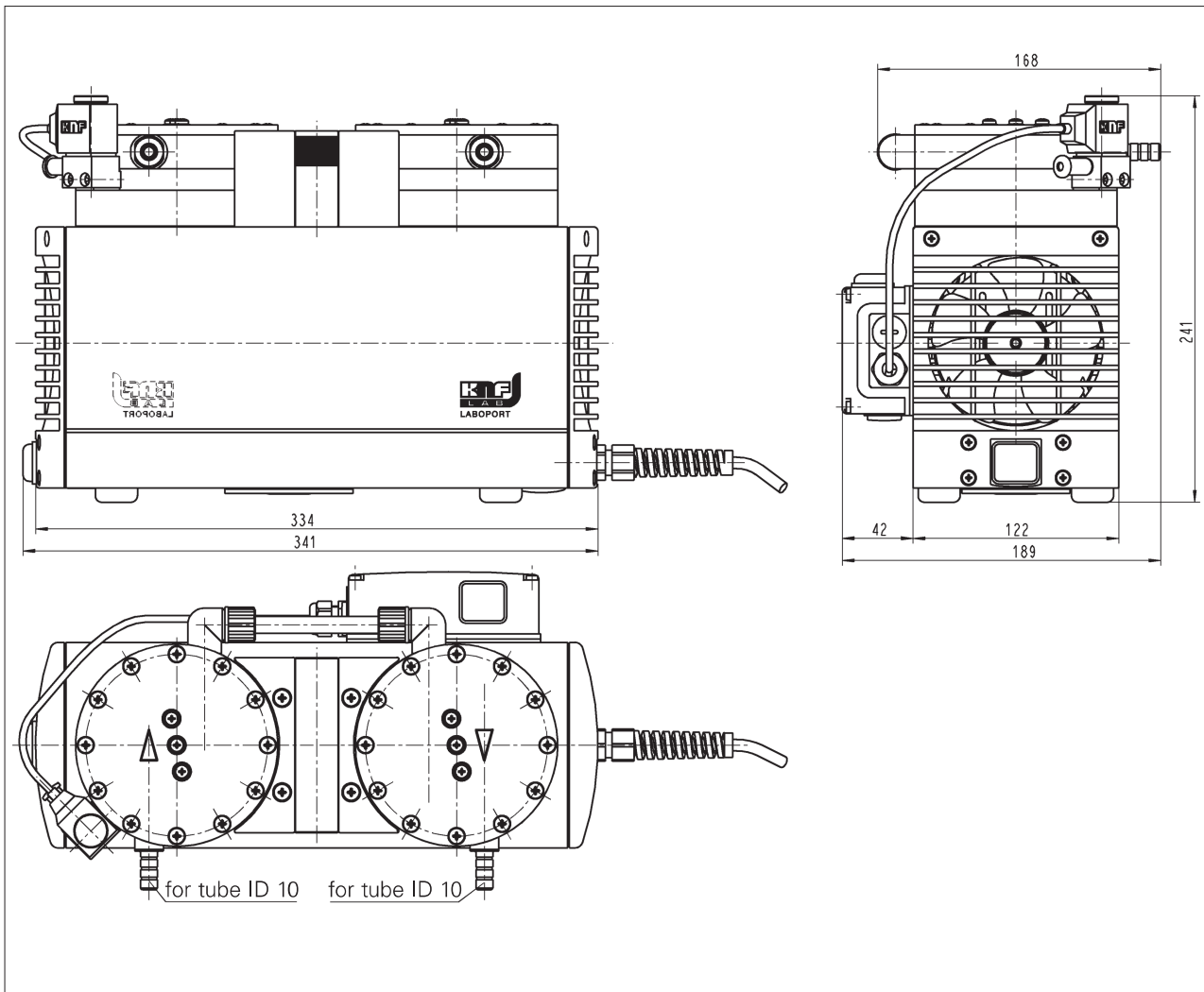
Dimensions (mm)
