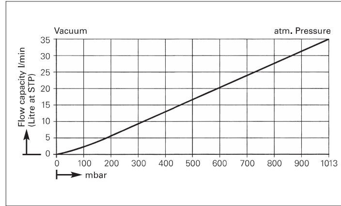
Performance characteristics
